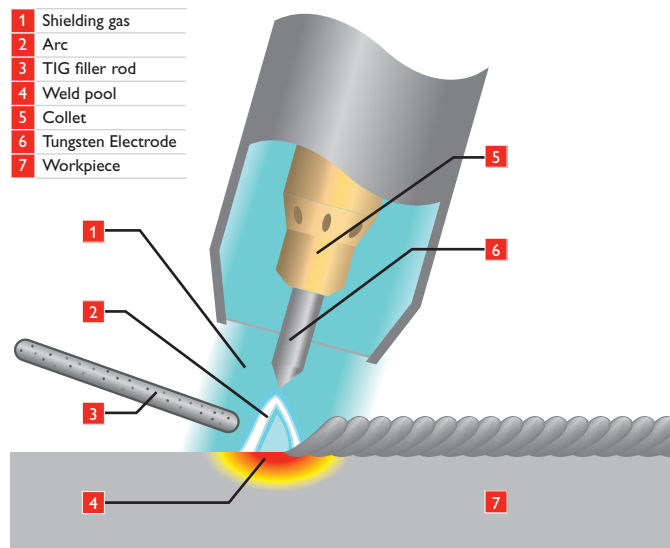
Schematic of the TIG welding process
